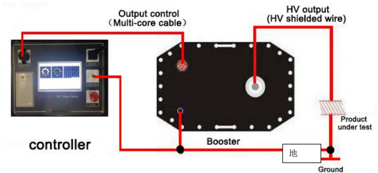
Figure 3 wiring diagram
